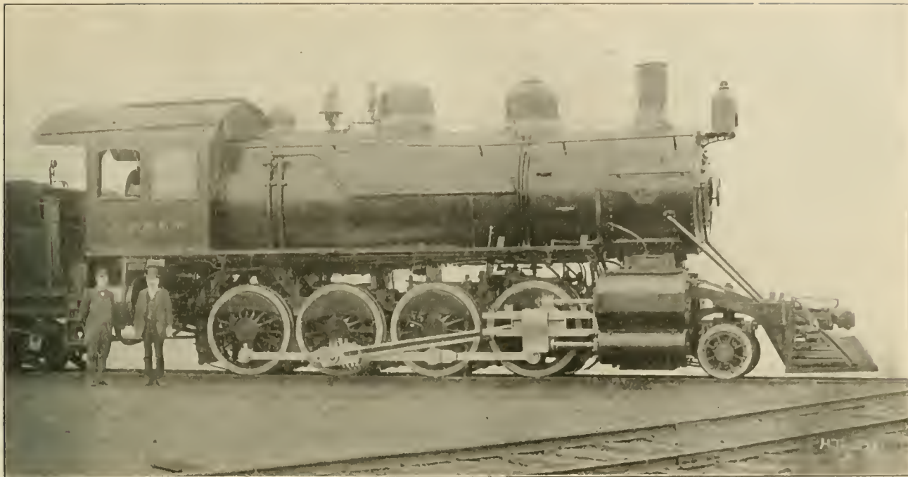
PLAYER-VAUCLAIN OIL-BURNING COMPOUND.
